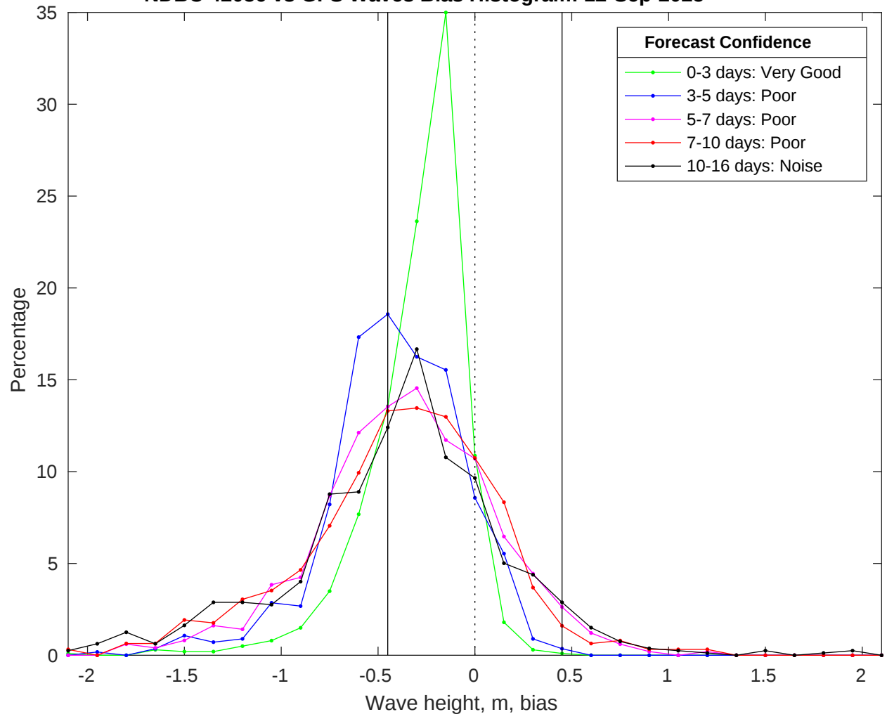
NDBC 42036 vs GFS Waves Bias Histogram: 12-Sep-2025
