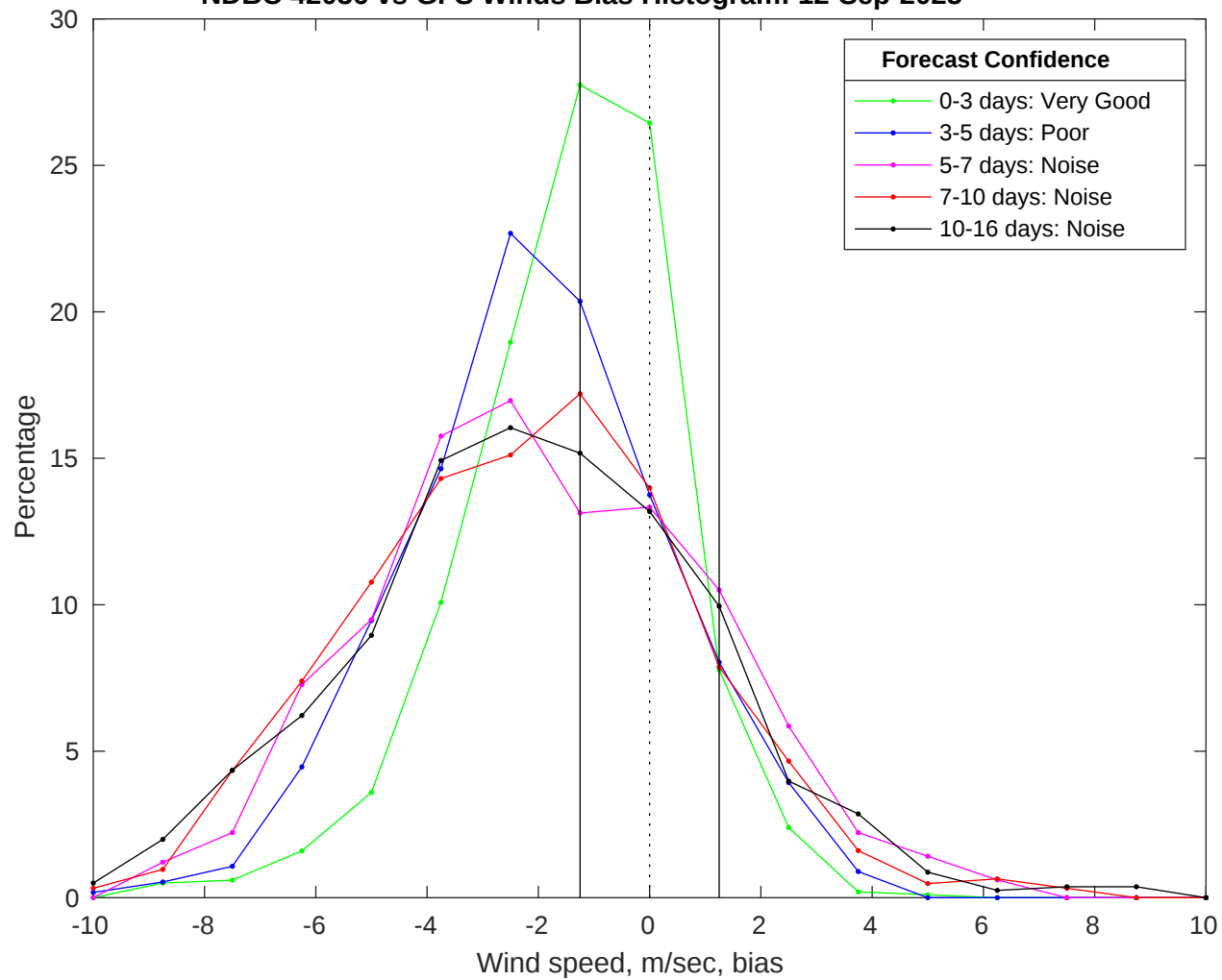
NDBC 42036 vs GFS Winds Bias Histogram: 12-Sep-2025
