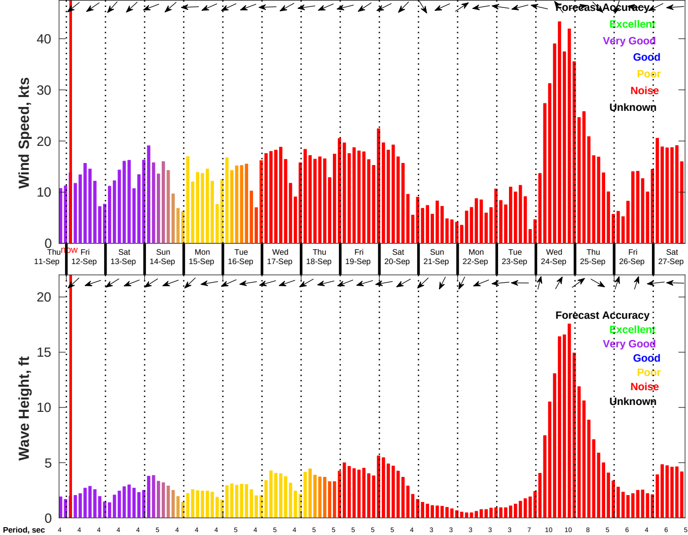
Wind & Wave Forecast for NDBC 42036 from 11-Sep-2025 19:00:00 to 27-Sep-2025 19:00:00
