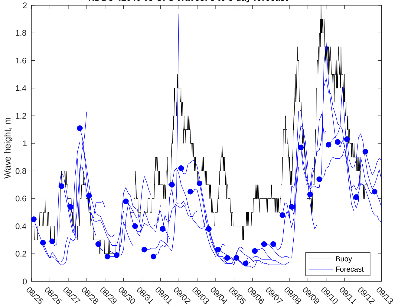
NDBC 42040 vs GFS Waves: 3 to 5 day forecast
