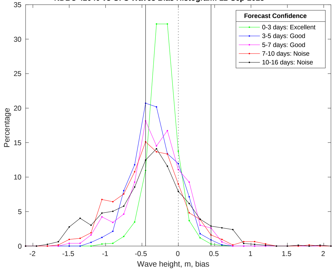
NDBC 42040 vs GFS Waves Bias Histogram: 12-Sep-2025
