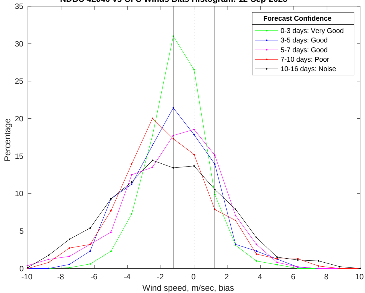
NDBC 42040 vs GFS Winds Bias Histogram: 12-Sep-2025
