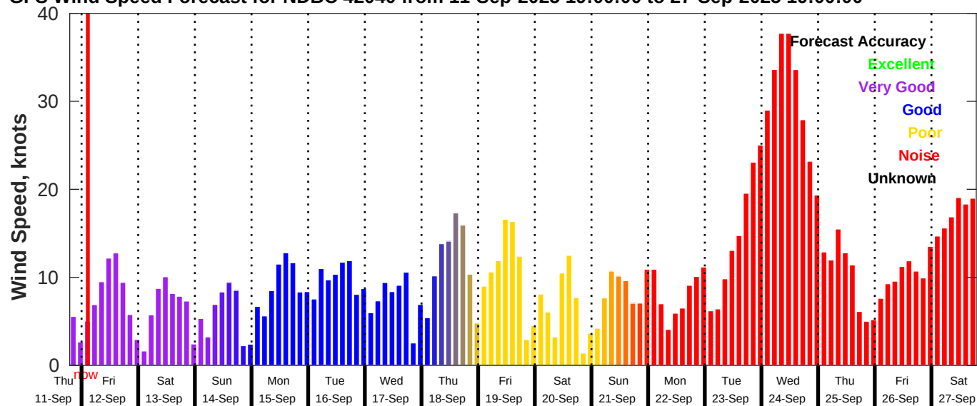
GFS Wind Speed Forecast for NDBC 42040 from 11-Sep-2025 19:00:00 to 27-Sep-2025 19:00:00
