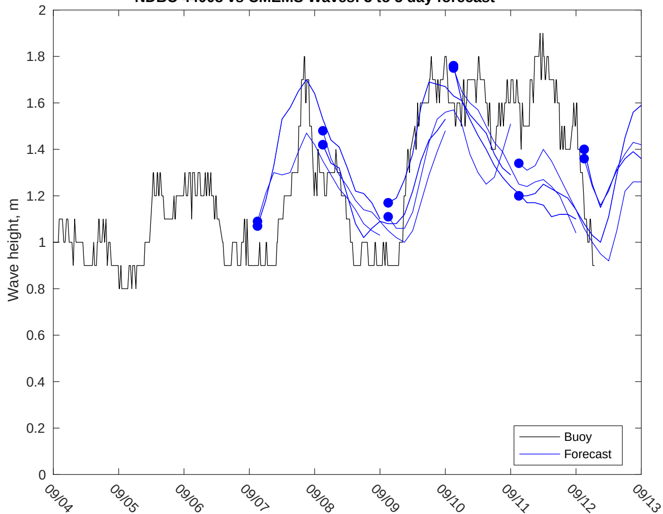
NDBC 44008 vs CMEMS Waves: 3 to 5 day forecast
