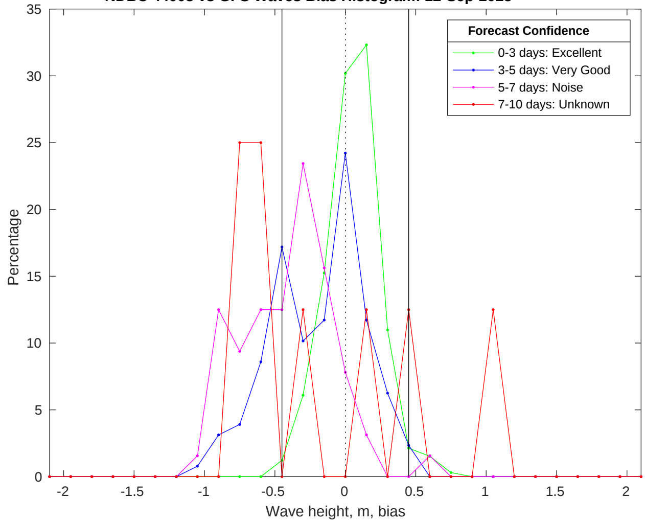
NDBC 44008 vs GFS Waves Bias Histogram: 12-Sep-2025
