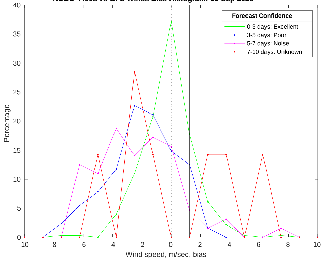
NDBC 44008 vs GFS Winds Bias Histogram: 12-Sep-2025
