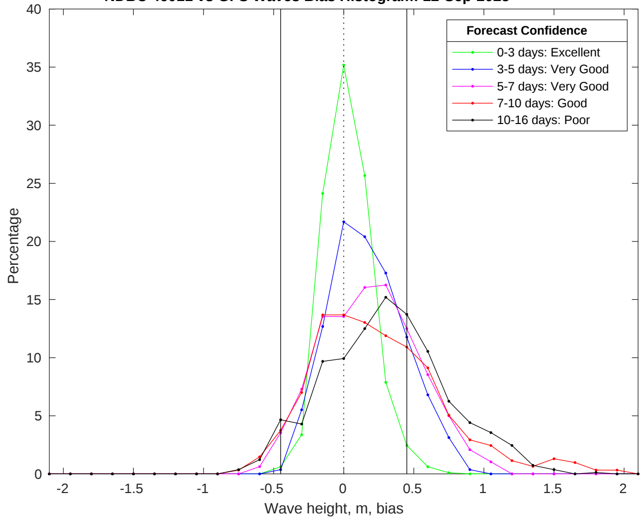
NDBC 46011 vs GFS Waves Bias Histogram: 12-Sep-2025
