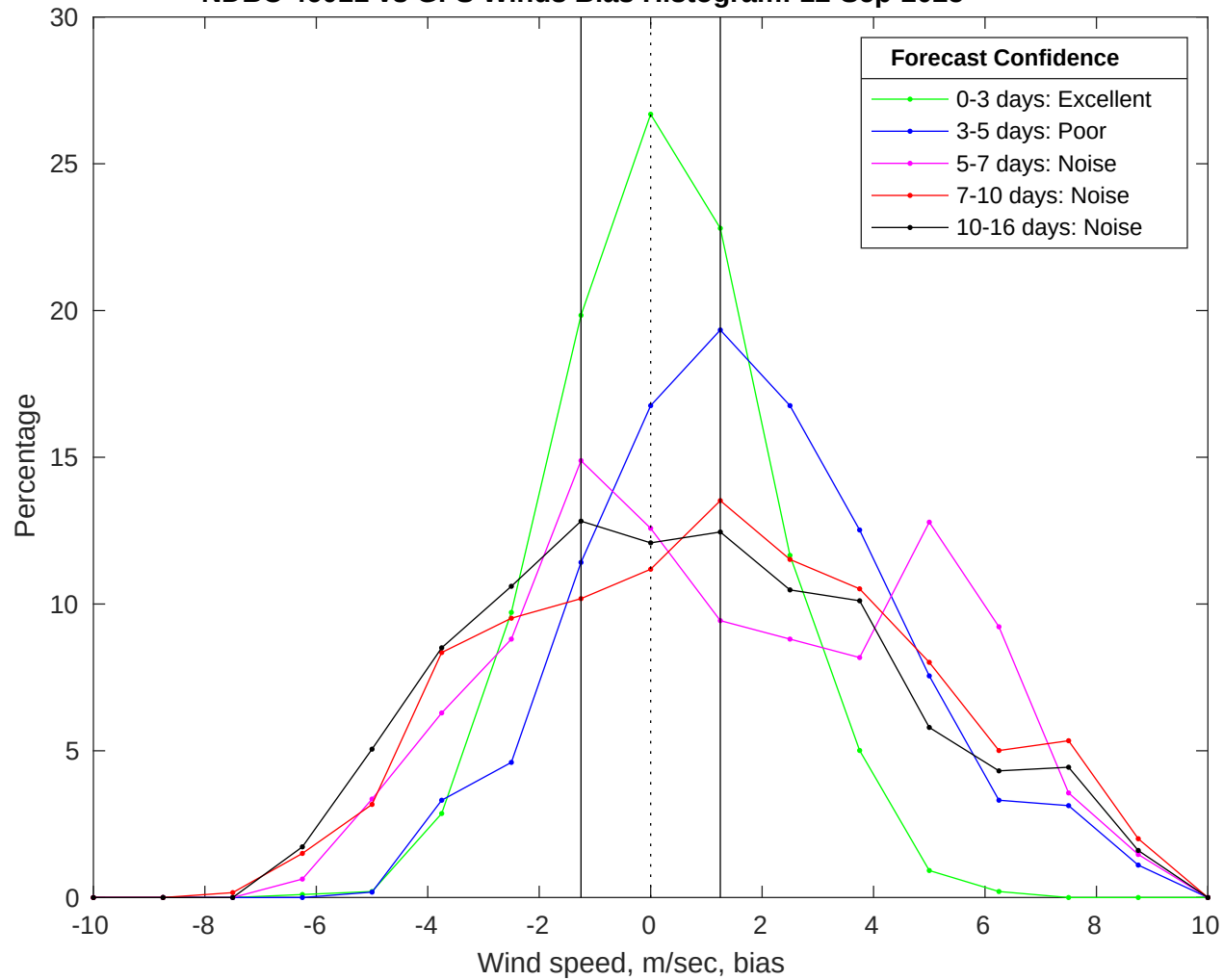
NDBC 46011 vs GFS Winds Bias Histogram: 12-Sep-2025
