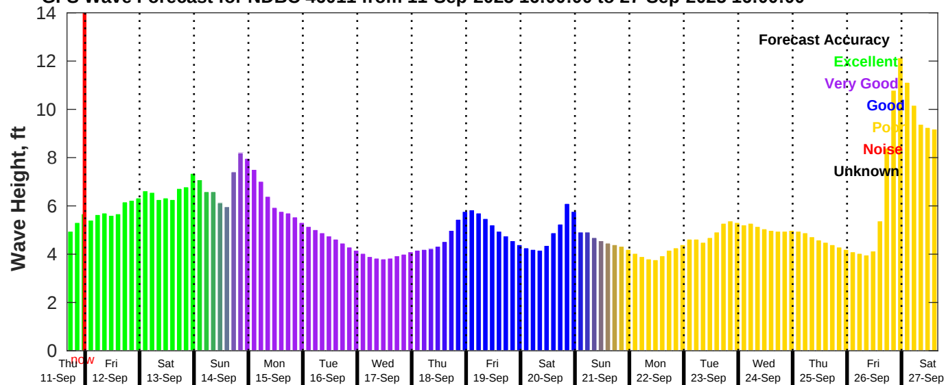
GFS Wave Forecast for NDBC 46011 from 11-Sep-2025 16:00:00 to 27-Sep-2025 16:00:00
