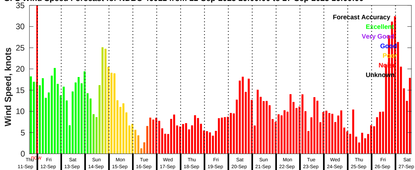
GFS Wind Speed Forecast for NDBC 46011 from 11-Sep-2025 16:00:00 to 27-Sep-2025 16:00:00
