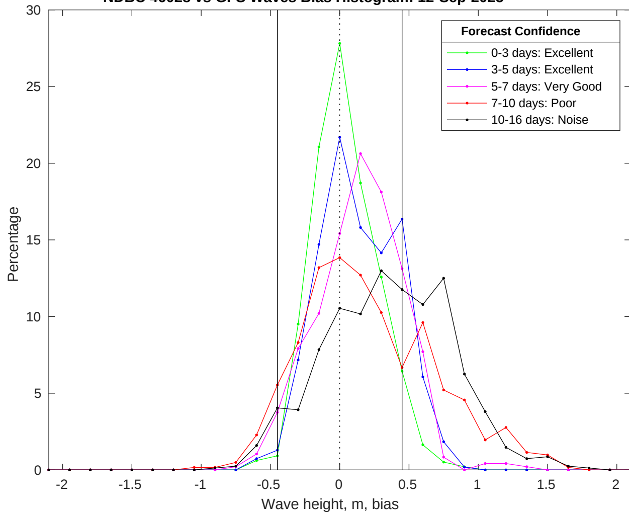
NDBC 46028 vs GFS Waves Bias Histogram: 12-Sep-2025
