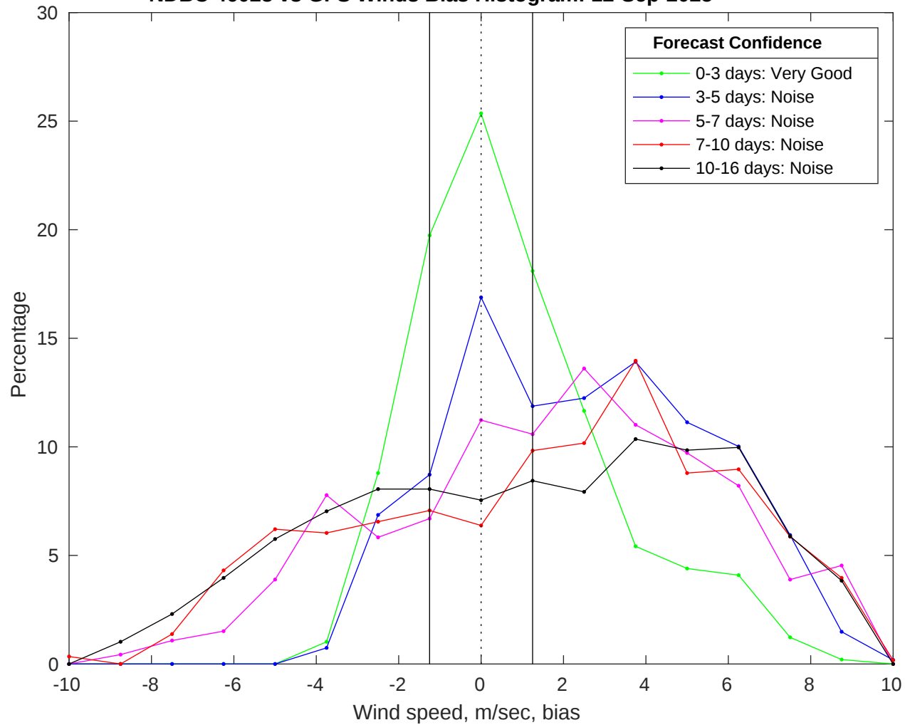
NDBC 46028 vs GFS Winds Bias Histogram: 12-Sep-2025
