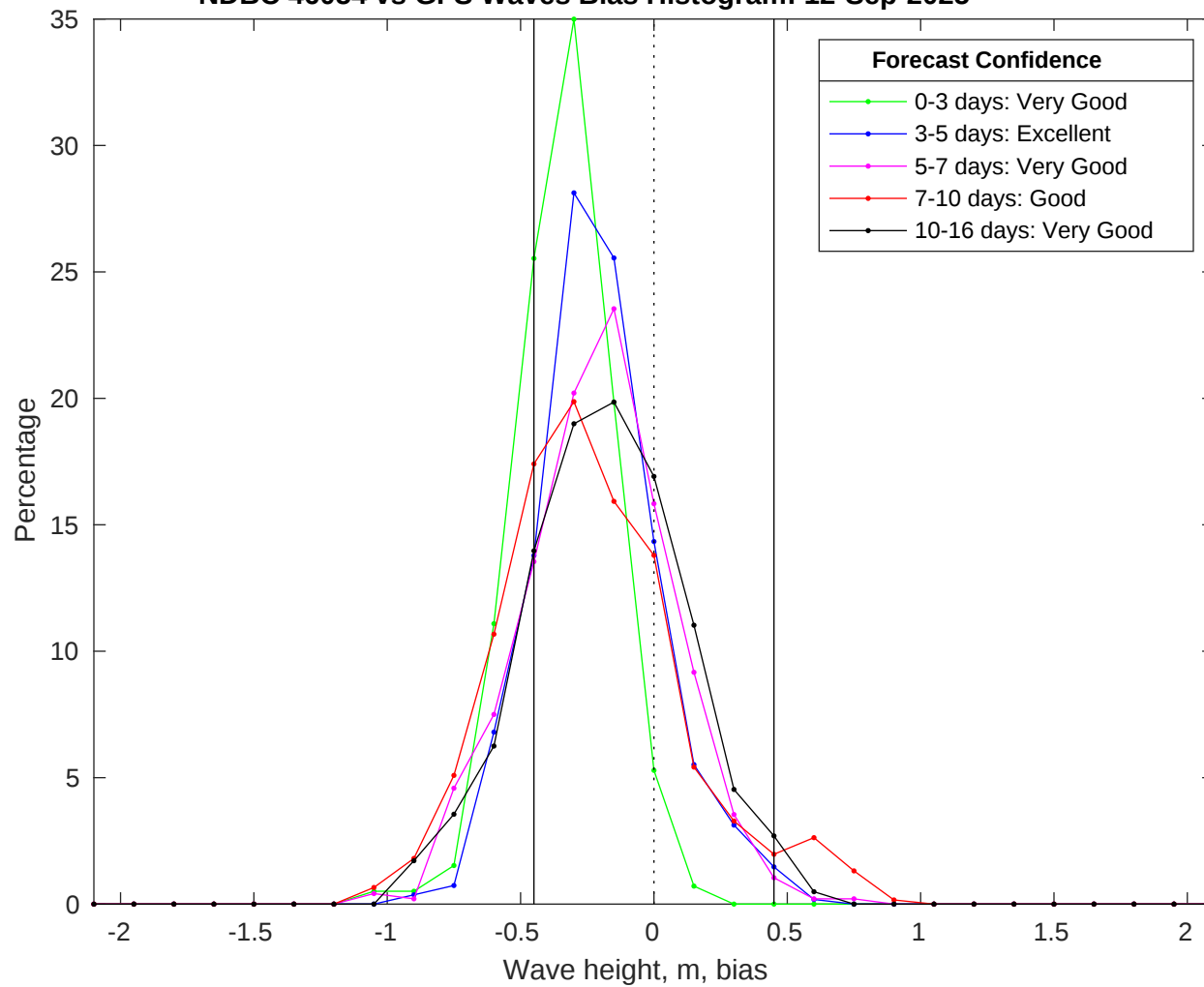
NDBC 46054 vs GFS Waves Bias Histogram: 12-Sep-2025
