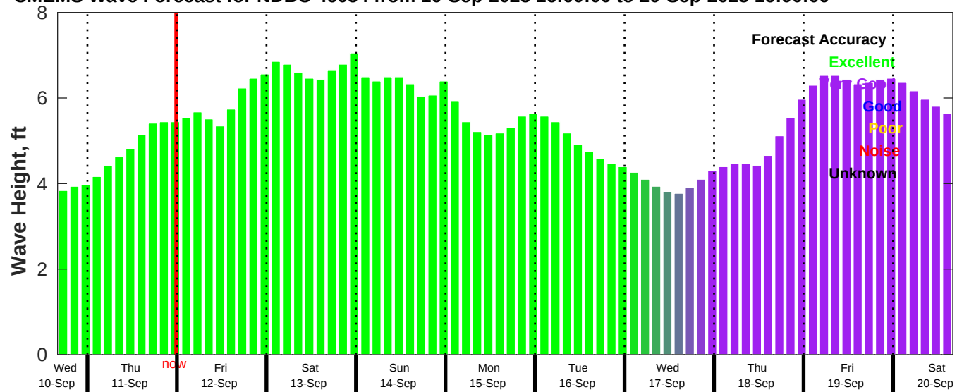
CMEMS Wave Forecast for NDBC 46054 from 10-Sep-2025 16:00:00 to 20-Sep-2025 16:00:00
