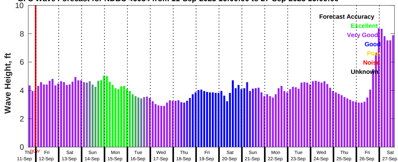
GFS Wave Forecast for NDBC 46054 from 11-Sep-2025 16:00:00 to 27-Sep-2025 16:00:00
