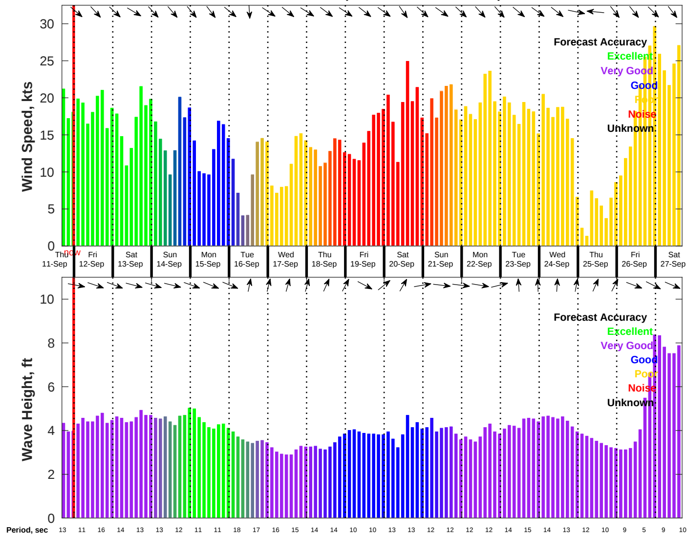
Wind & Wave Forecast for NDBC 46054 from 11-Sep-2025 16:00:00 to 27-Sep-2025 16:00:00
