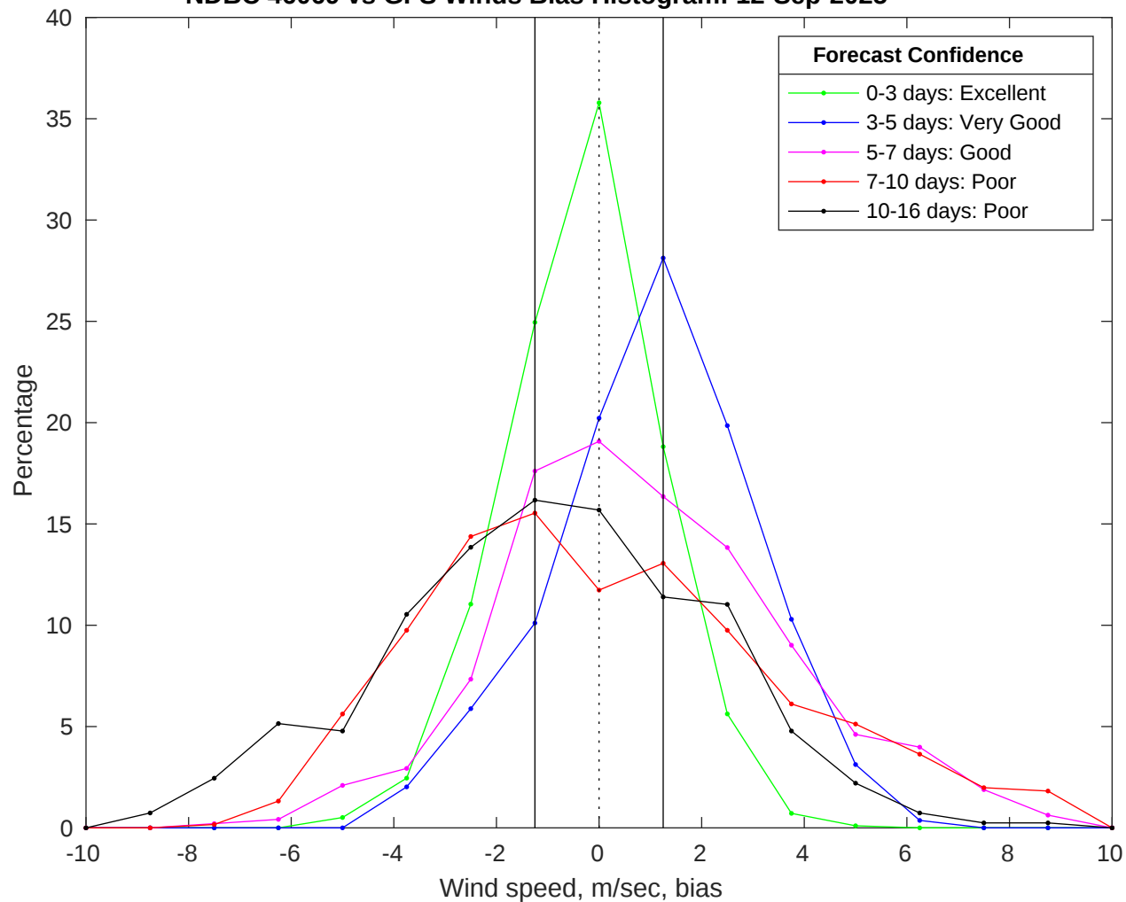
NDBC 46069 vs GFS Winds Bias Histogram: 12-Sep-2025
