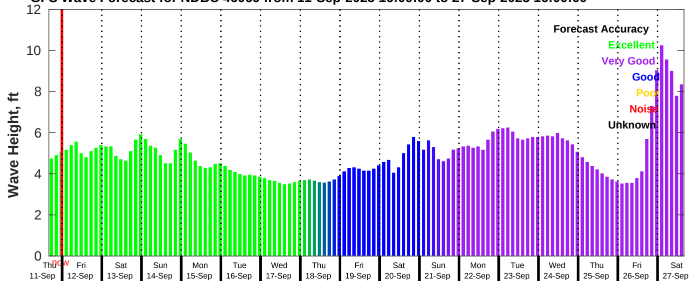
GFS Wave Forecast for NDBC 46069 from 11-Sep-2025 16:00:00 to 27-Sep-2025 16:00:00
