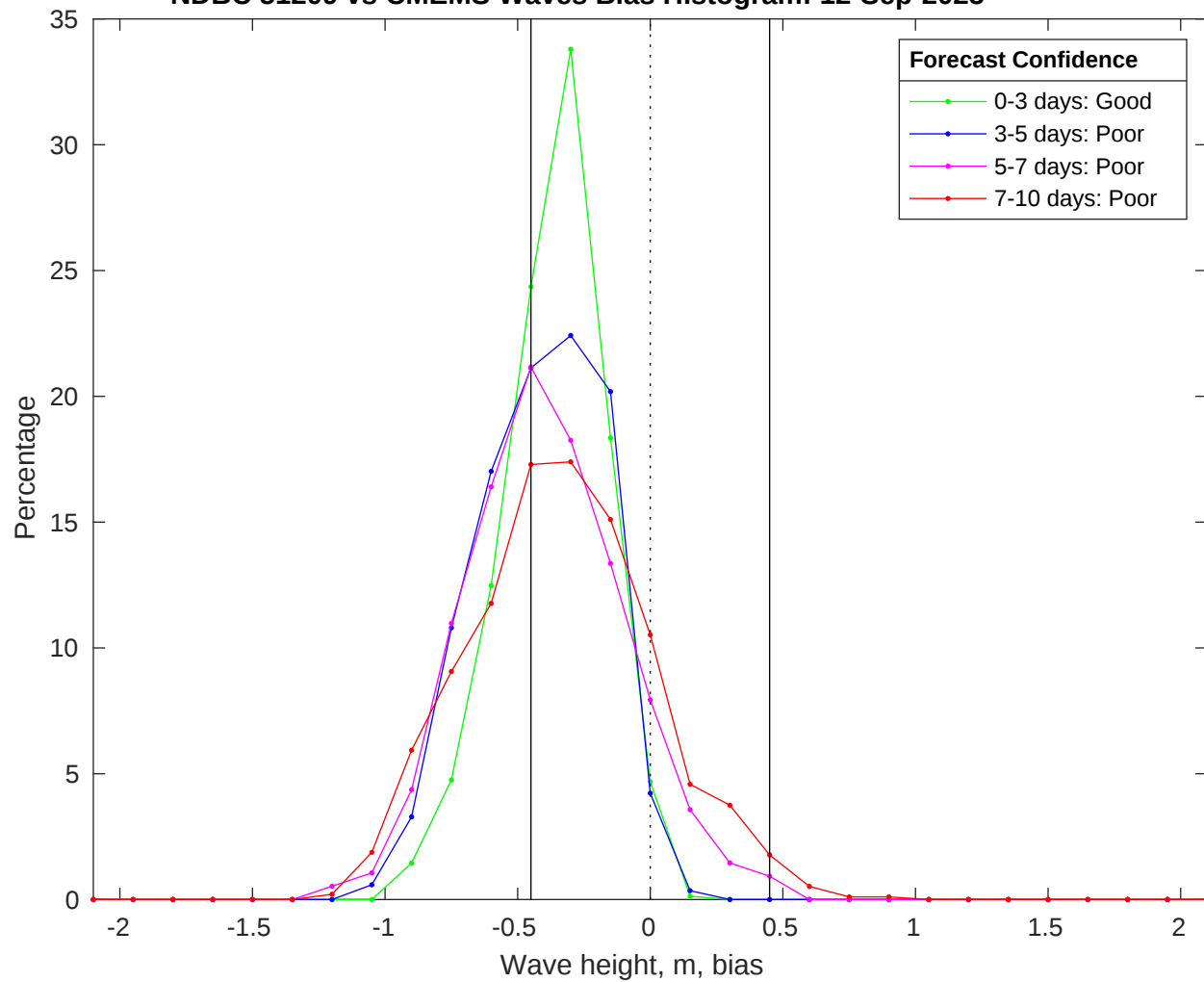
NDBC 51209 vs CMEMS Waves Bias Histogram: 12-Sep-2025
