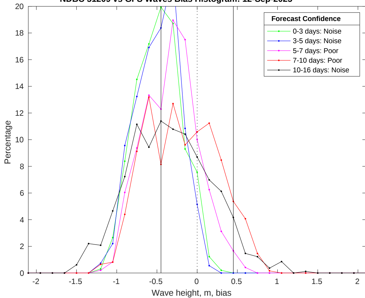
NDBC 51209 vs GFS Waves Bias Histogram: 12-Sep-2025
