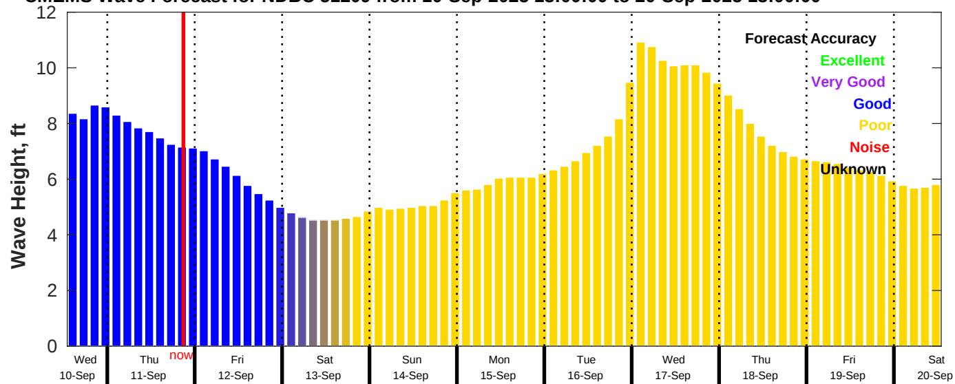
CMEMS Wave Forecast for NDBC 51209 from 10-Sep-2025 13:00:00 to 20-Sep-2025 13:00:00
