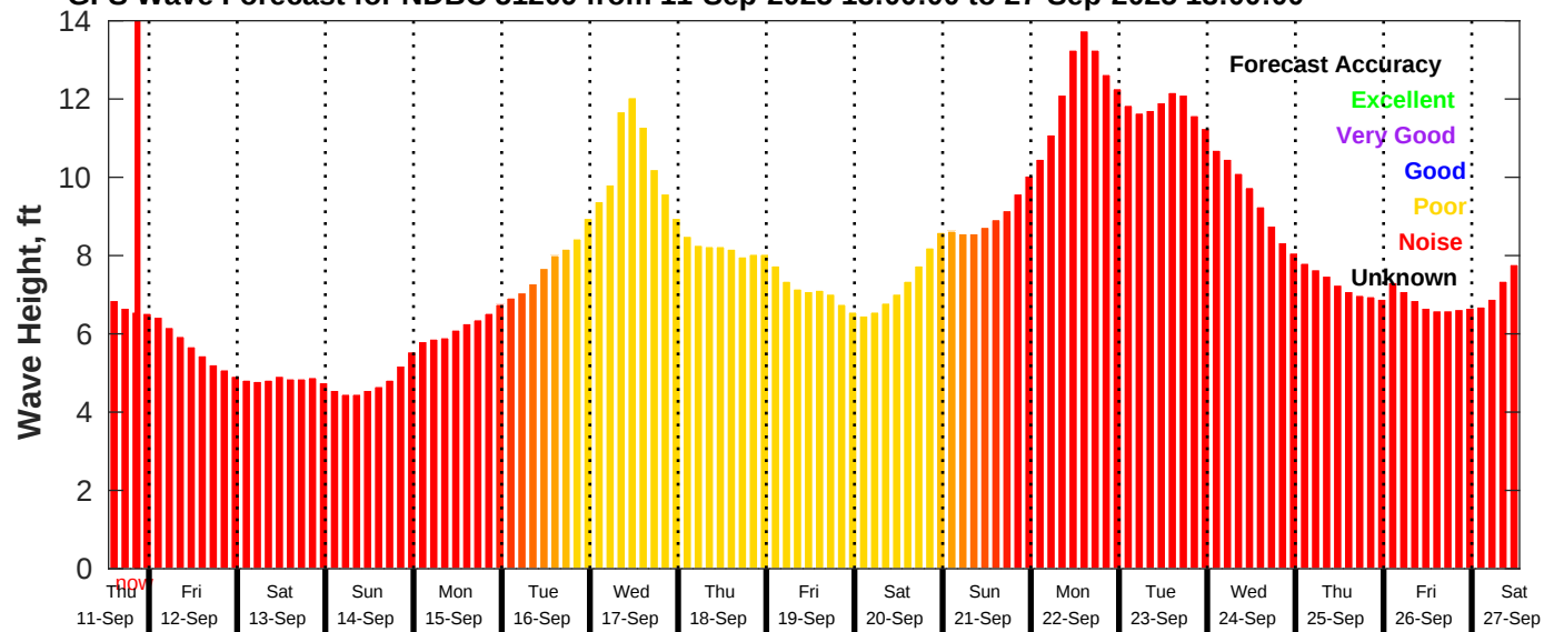
GFS Wave Forecast for NDBC 51209 from 11-Sep-2025 13:00:00 to 27-Sep-2025 13:00:00
