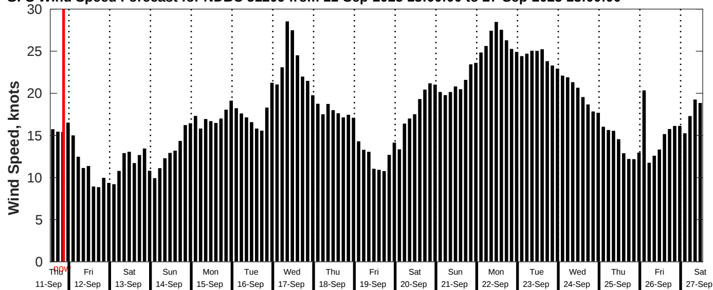
GFS Wind Speed Forecast for NDBC 51209 from 11-Sep-2025 13:00:00 to 27-Sep-2025 13:00:00
