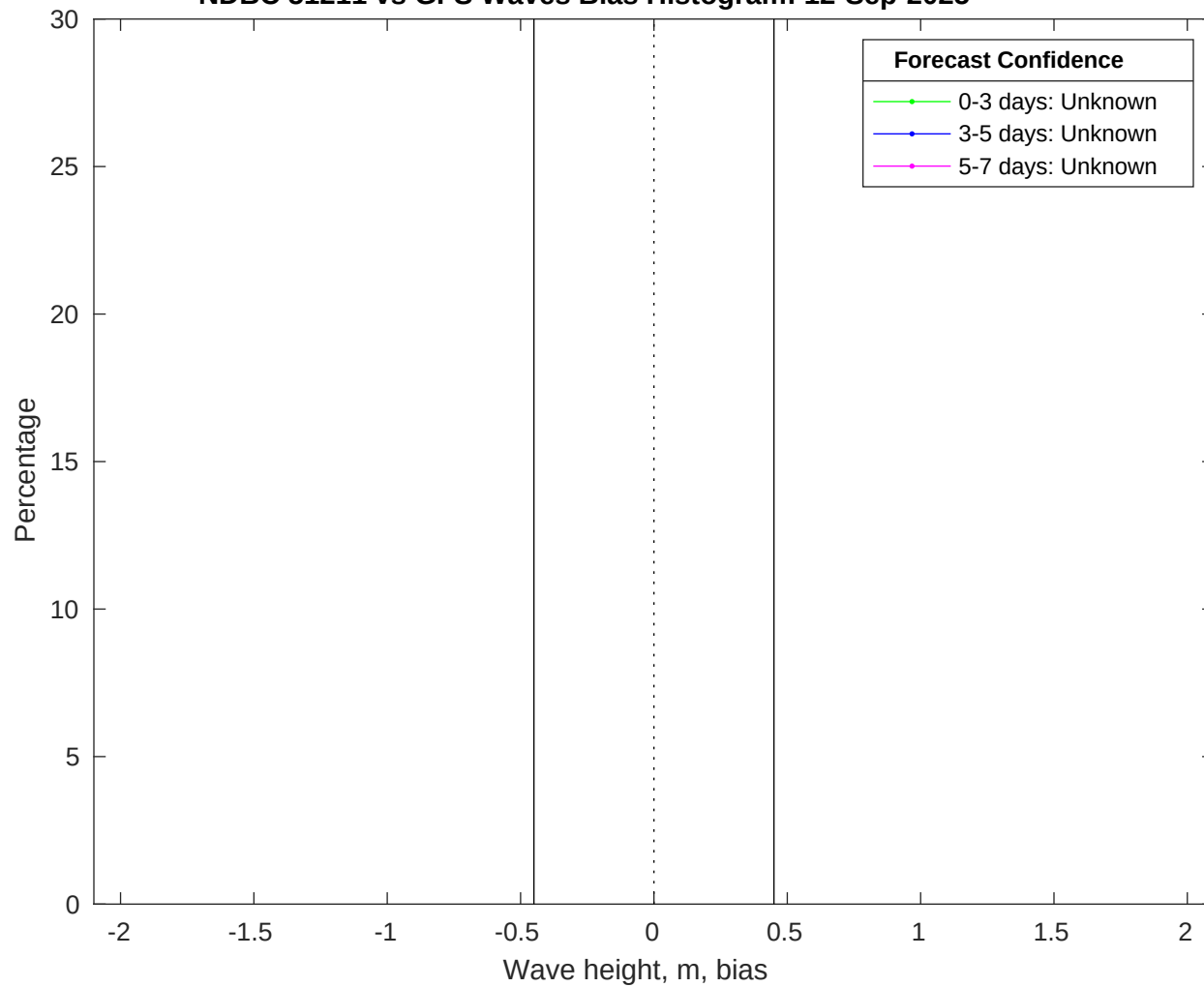
NDBC 51211 vs GFS Waves Bias Histogram: 12-Sep-2025
