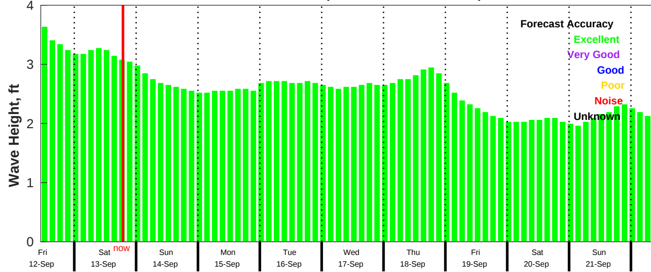
CMEMS Wave Forecast for NDBC 52211 from 11-Sep-2025 11:00:00 to 21-Sep-2025 11:00:00
