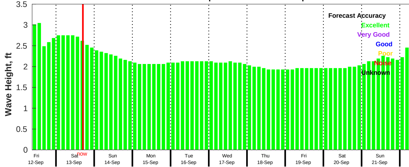
CMEMS Wave Forecast for NDBC 52212 from 11-Sep-2025 09:00:00 to 21-Sep-2025 09:00:00
