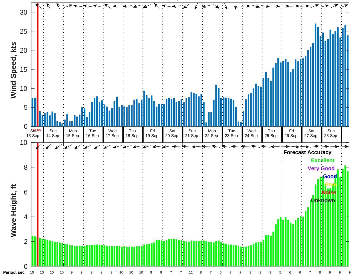
Wind & Wave Forecast for NDBC 52212 from 12-Sep-2025 09:00:00 to 28-Sep-2025 09:00:00
