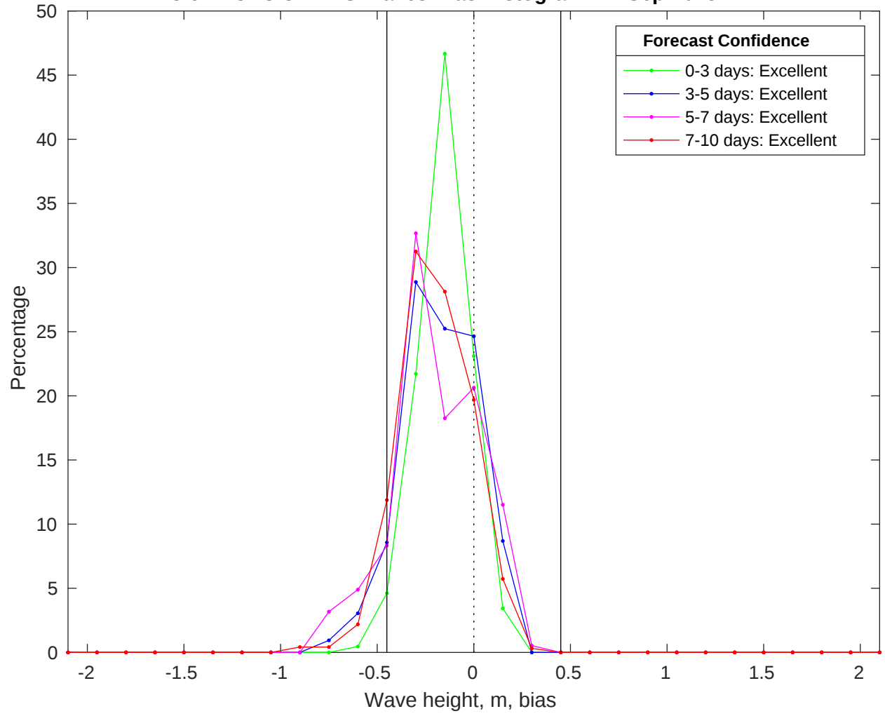
NDBC 52213 vs CMEMS Waves Bias Histogram: 12-Sep-2025
