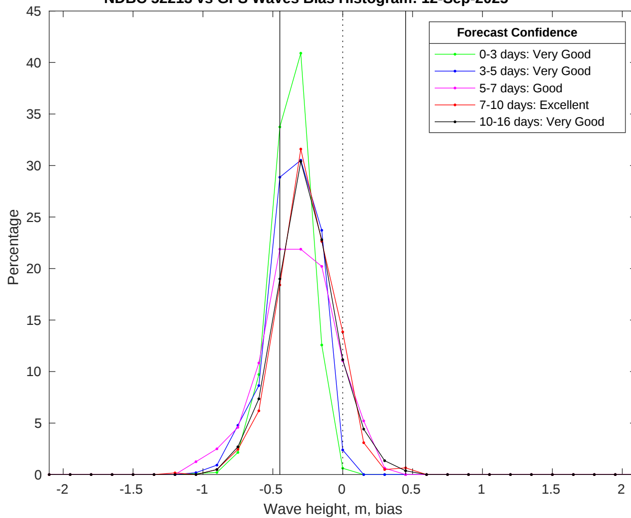
NDBC 52213 vs GFS Waves Bias Histogram: 12-Sep-2025
