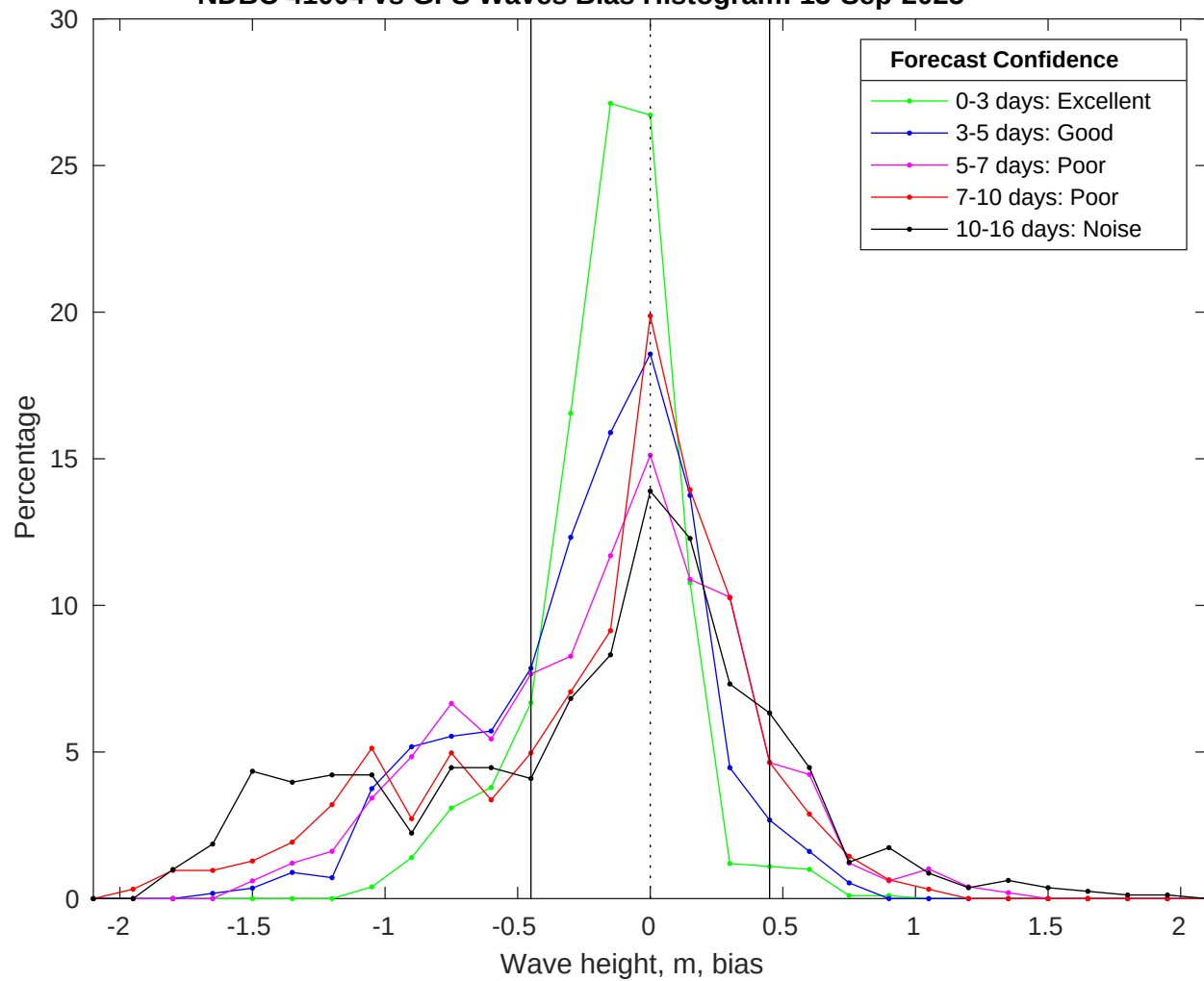
NDBC 41004 vs GFS Waves Bias Histogram: 13-Sep-2025
