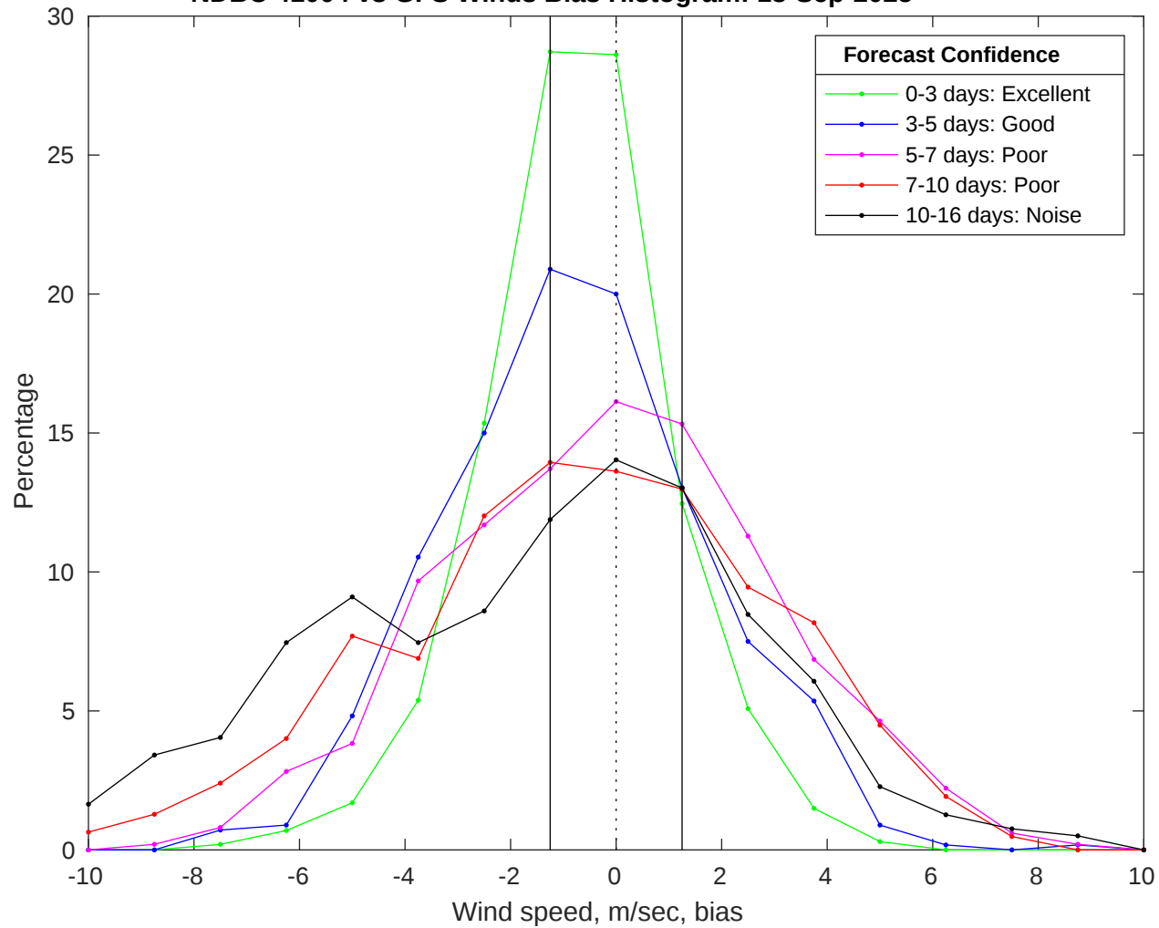
NDBC 41004 vs GFS Winds Bias Histogram: 13-Sep-2025
