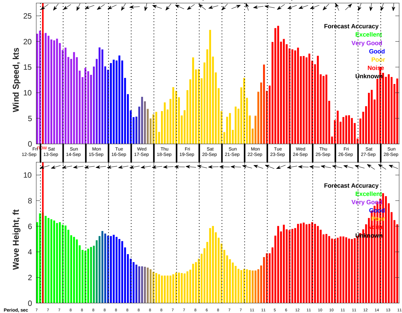
Wind & Wave Forecast for NDBC 41004 from 12-Sep-2025 19:00:00 to 28-Sep-2025 19:00:00
