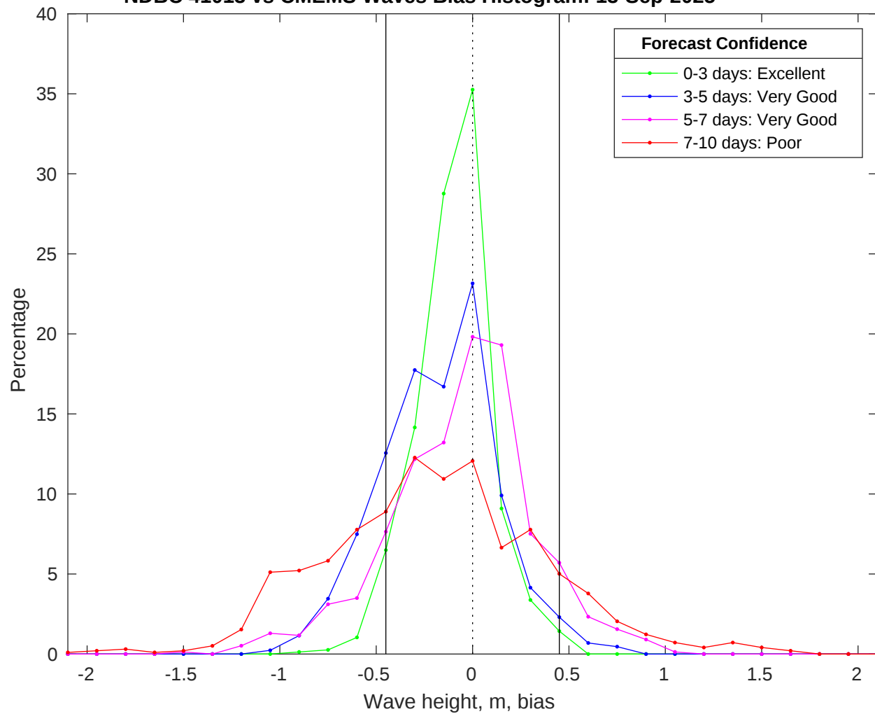
NDBC 41013 vs CMEMS Waves Bias Histogram: 13-Sep-2025
