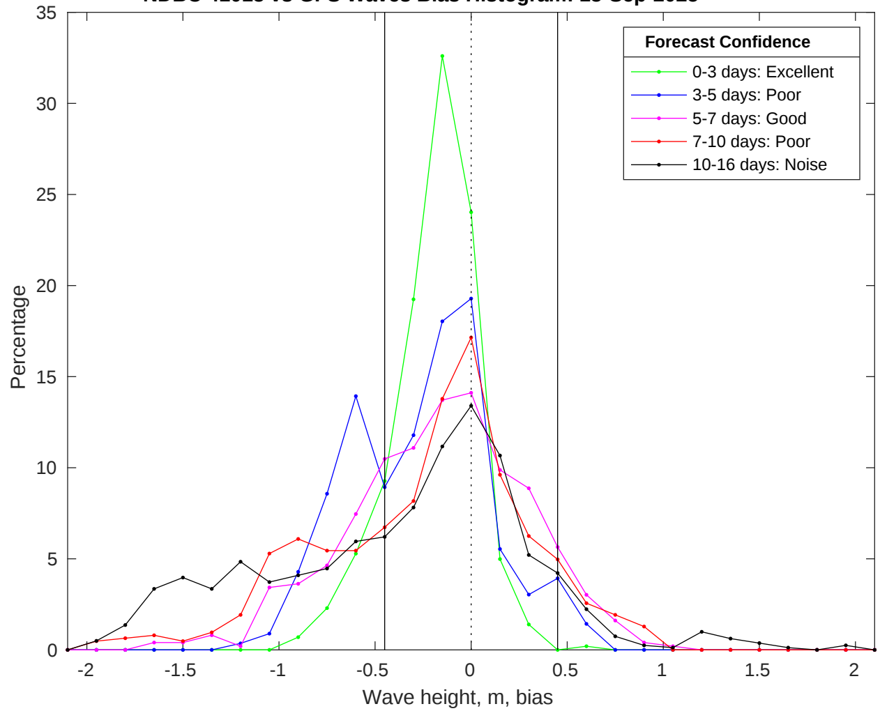
NDBC 41013 vs GFS Waves Bias Histogram: 13-Sep-2025
