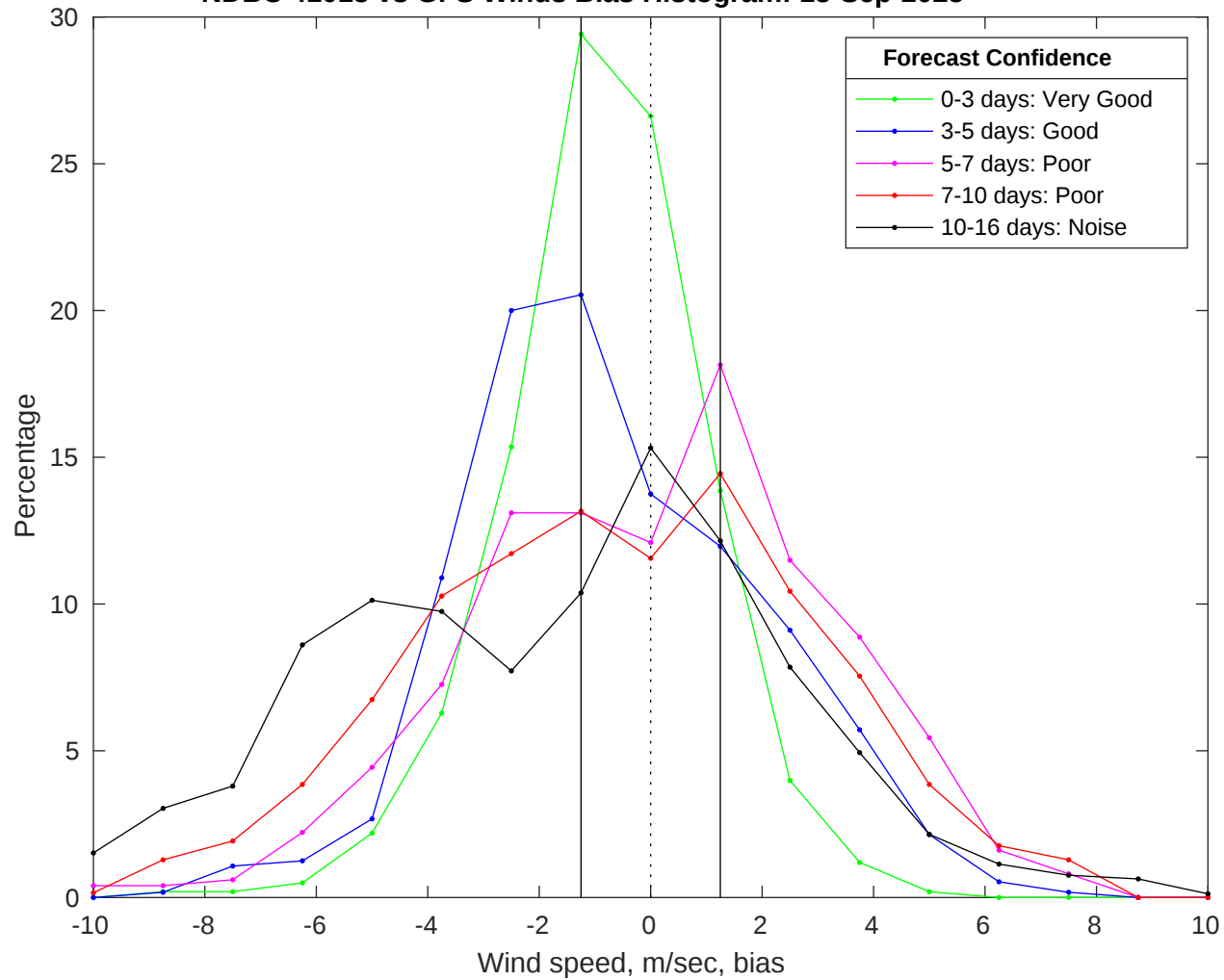
NDBC 41013 vs GFS Winds Bias Histogram: 13-Sep-2025
