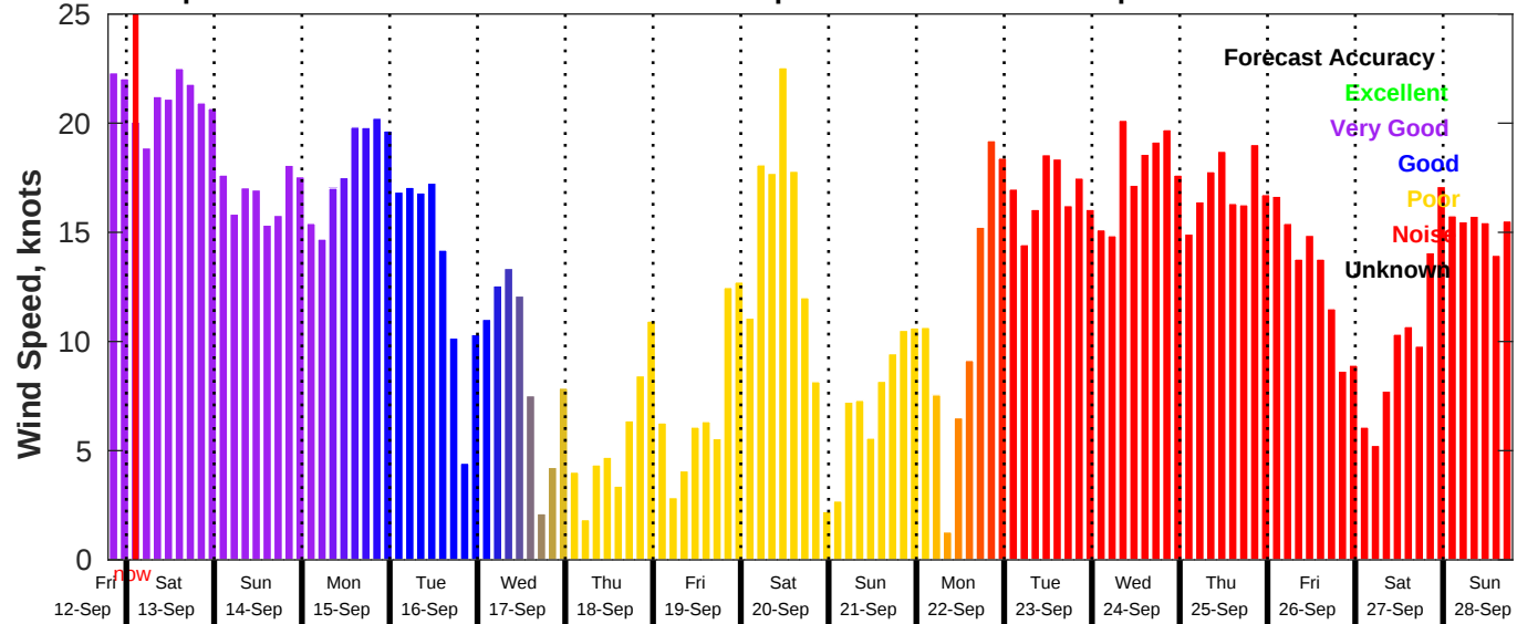
GFS Wind Speed Forecast for NDBC 41013 from 12-Sep-2025 19:00:00 to 28-Sep-2025 19:00:00
