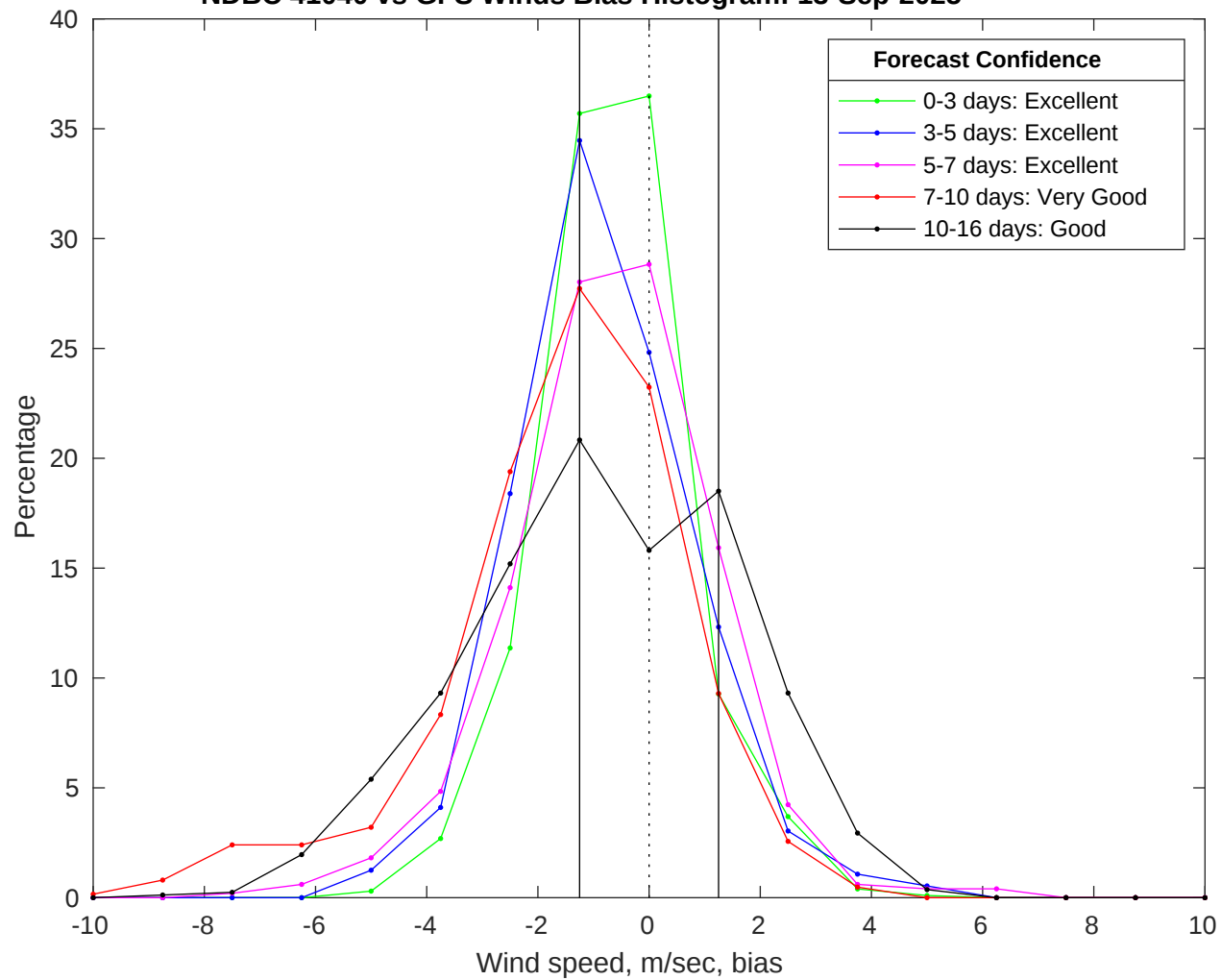
NDBC 41040 vs GFS Winds Bias Histogram: 13-Sep-2025
