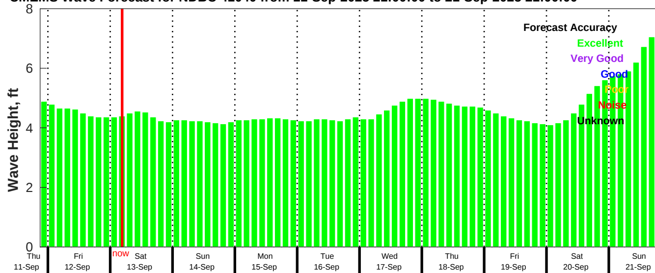
CEEMS Wave Forecast for NDBC 41040 from 11-Sep-2025 21:00:00 to 21-Sep-2025 21:00:00
