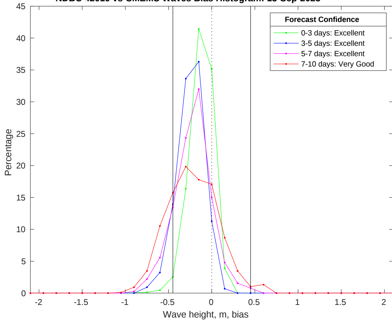
NDBC 42019 vs CMEMS Waves Bias Histogram: 13-Sep-2025
