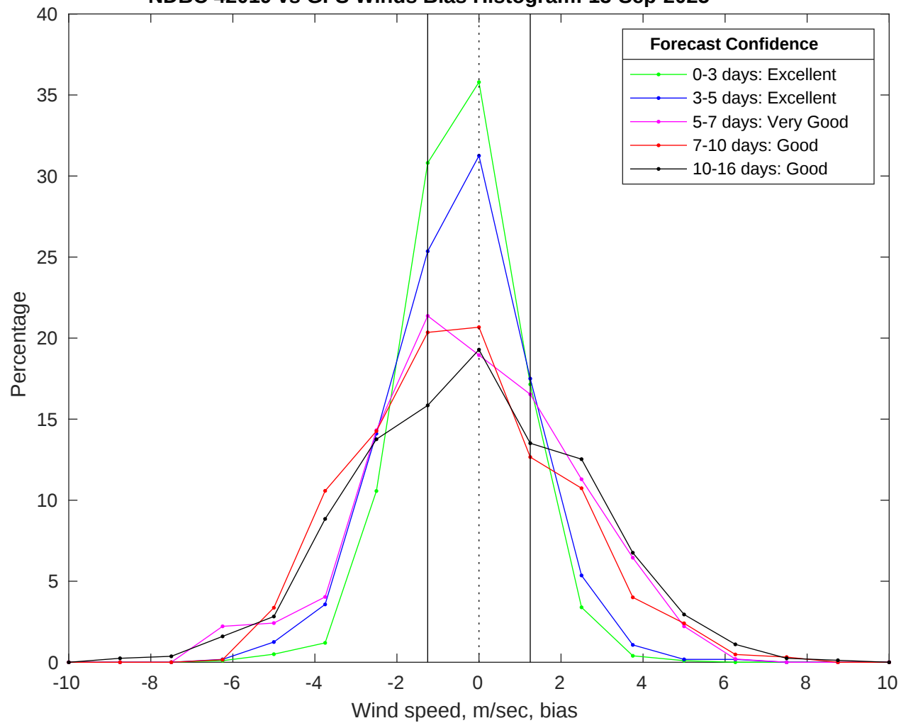
NDBC 42019 vs GFS Winds Bias Histogram: 13-Sep-2025
