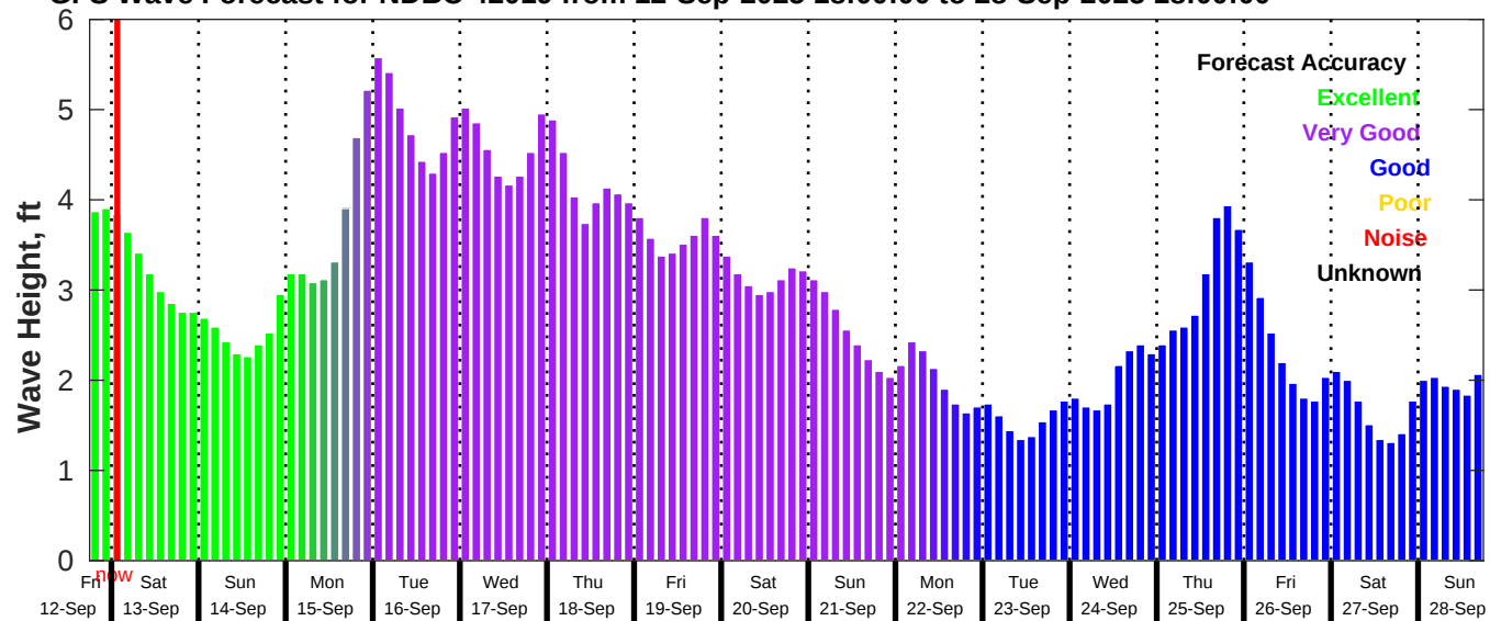
GFS Wave Forecast for NDBC 42019 from 12-Sep-2025 18:00:00 to 28-Sep-2025 18:00:00
