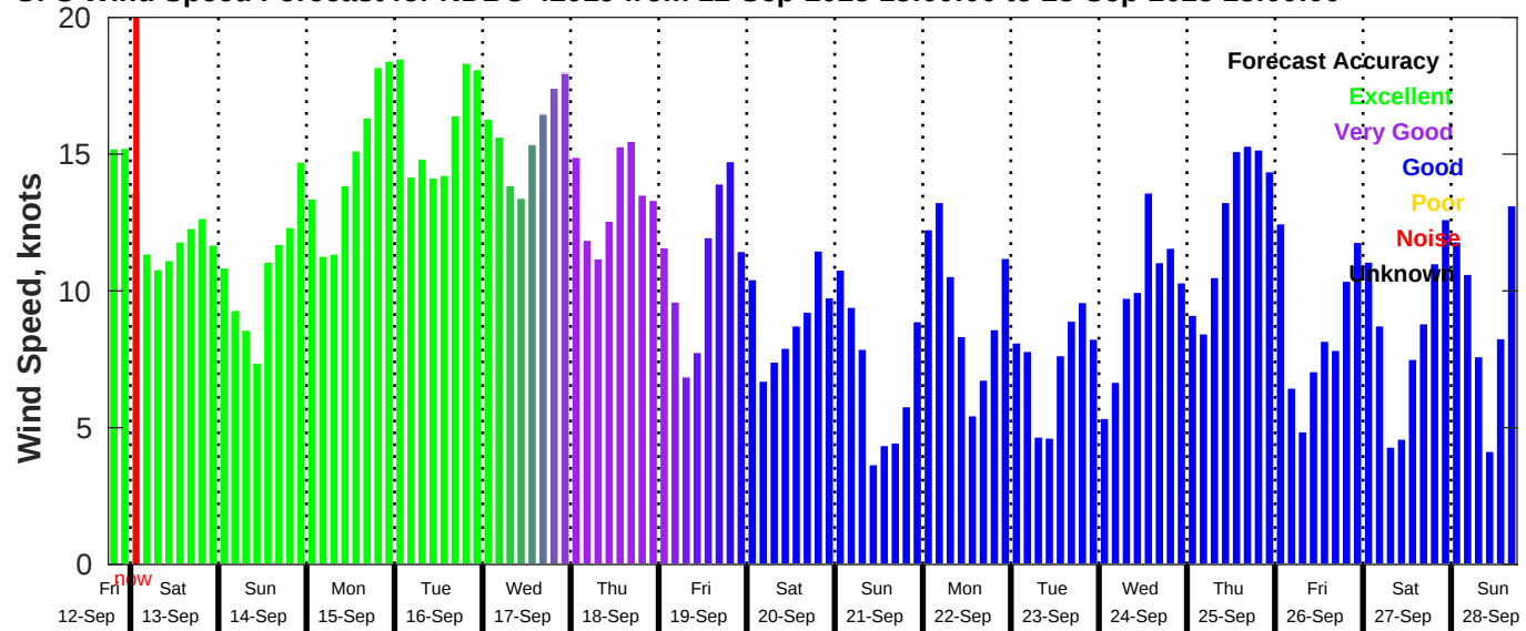
GFS Wind Speed Forecast for NDBC 42019 from 12-Sep-2025 18:00:00 to 28-Sep-2025 18:00:00
