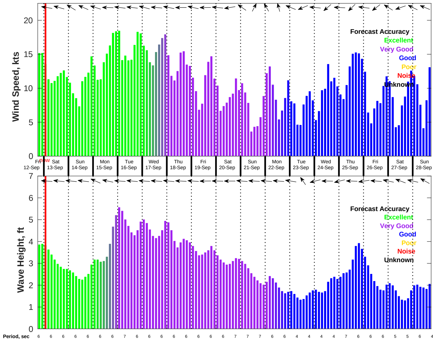
Wind & Wave Forecast for NDBC 42019 from 12-Sep-2025 18:00:00 to 28-Sep-2025 18:00:00
