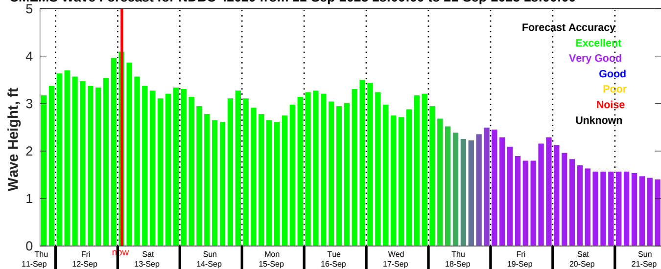
CMEMS Wave Forecast for NDBC 42020 from 11-Sep-2025 18:00:00 to 21-Sep-2025 18:00:00
