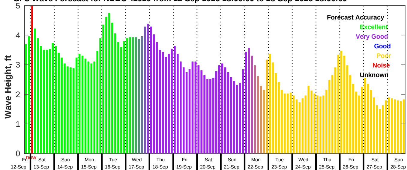
GFS Wave Forecast for NDBC 42020 from 12-Sep-2025 18:00:00 to 28-Sep-2025 18:00:00
