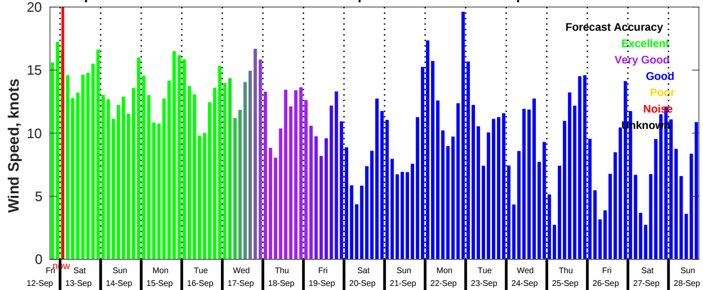
GFS Wind Speed Forecast for NDBC 42020 from 12-Sep-2025 18:00:00 to 28-Sep-2025 18:00:00
